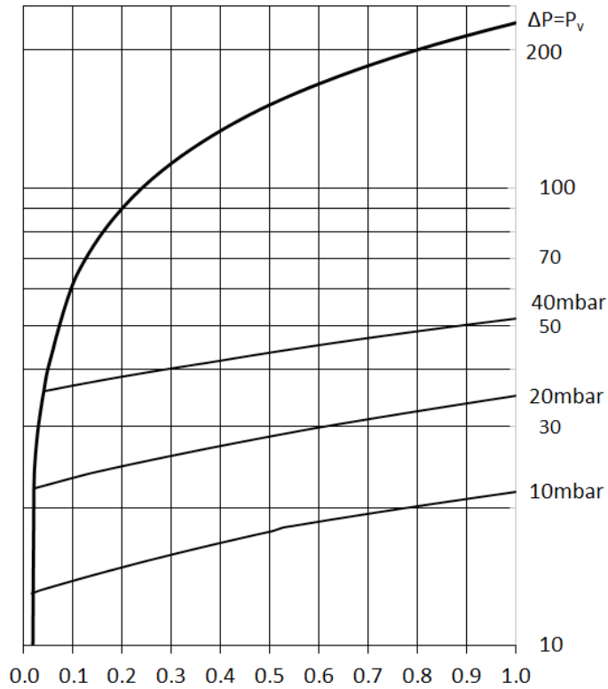
Flow diagram for air (20 °C / 68 °F)
